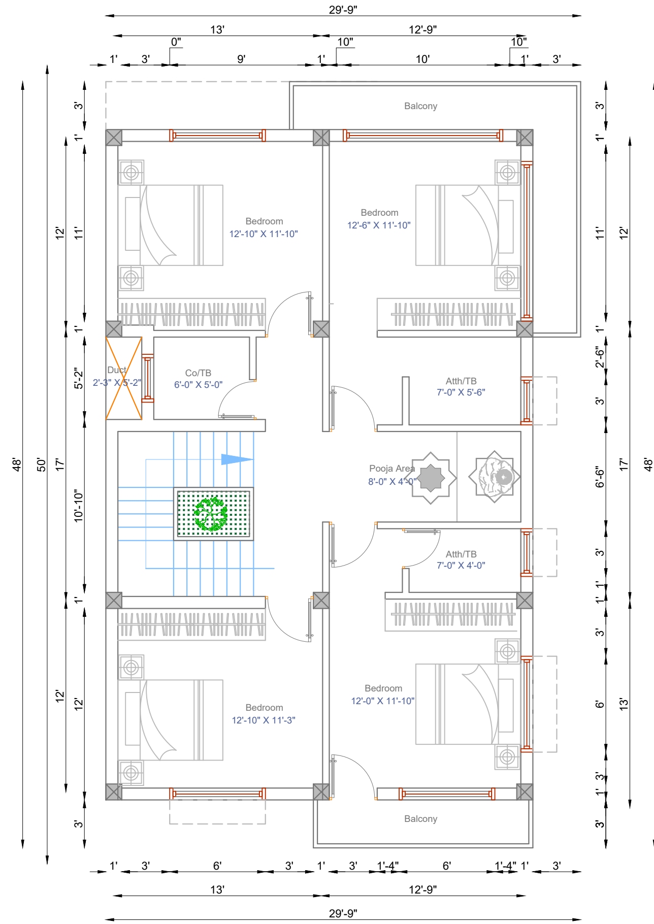
FIRST FLOOR PLAN Plinth Area: 1123.50 Sq.Ft
