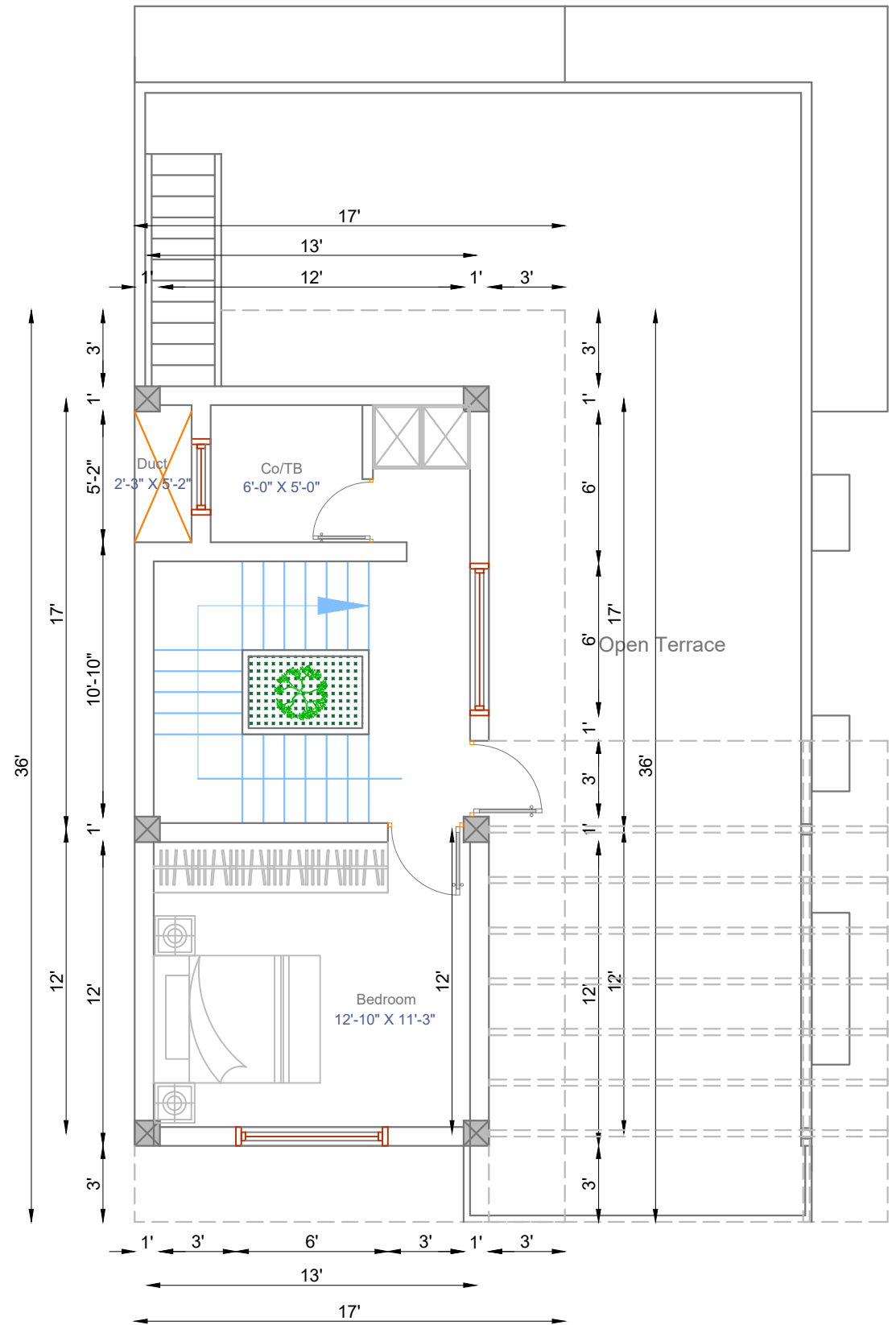
SECOND FLOOR PLAN Plinth Area: 420.00 Sq.Ft
